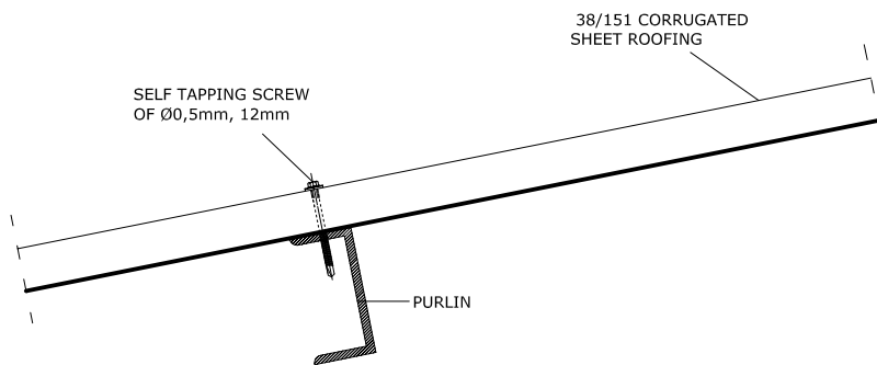
FIXING TO PURLIN
