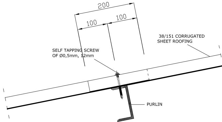
INSTALLATION DETAIL OF SPLICE
