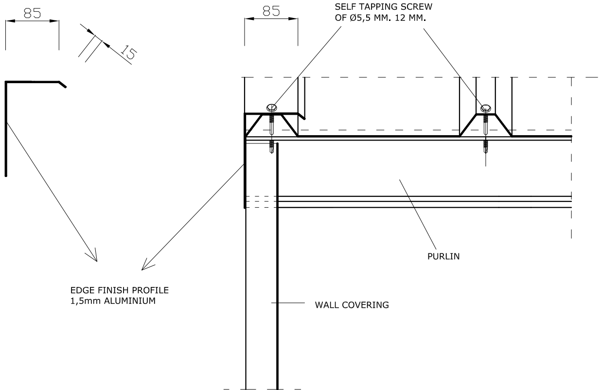
BUILDING WITHOUT EAVES
