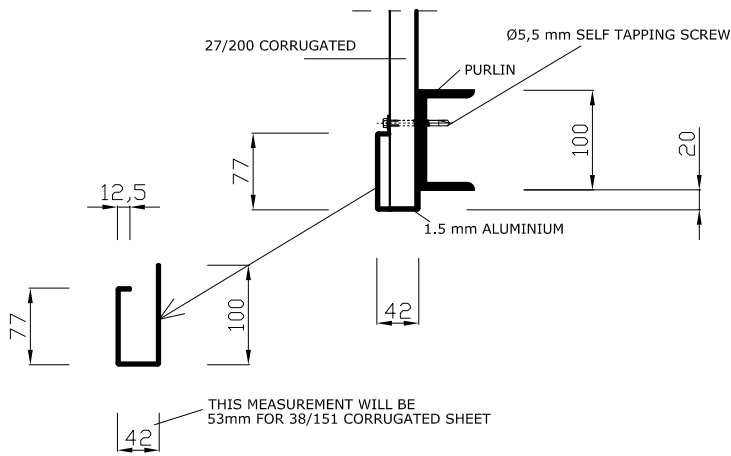
4-4 DETAIL
