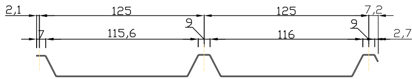
PANEL 250 CROSS SECTION
