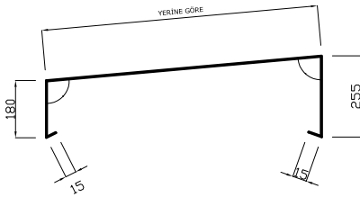
NO15 : PARAPET SHEET
