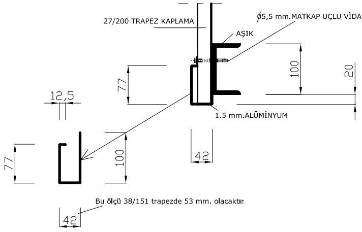
4-4 DETAYI
